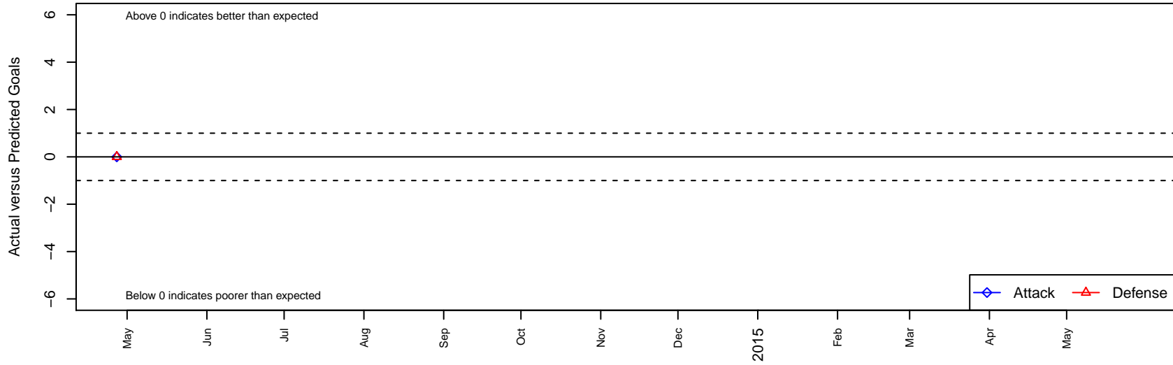
Oxnard AC Blue B98 Dots are actual minus expected GF (blue circles) and GA (red triangles). Blue line is smoothed change in attack strength. Red is smoothed change in defense strength.
